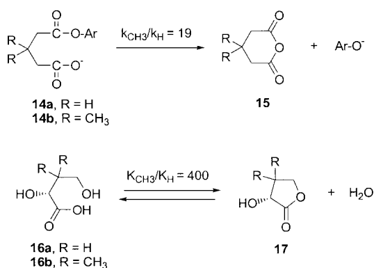
Figure 3. Effects of geminal dimethyl groups on cyclization reactions.
