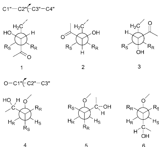
Figure 2. Newman projections of the low-energy rotamers about the C2''–C3'' and C1''–C2'' bonds of coenzyme A.
