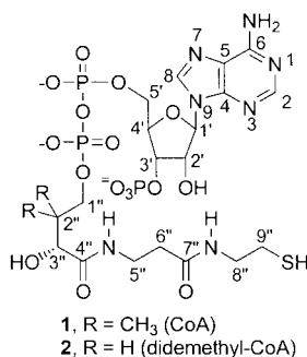
Figure 1. Structures of coenzyme A and a didemethyl analogue.
